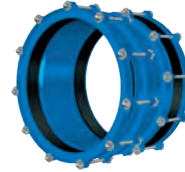
Series 8004 Fabricated universal flange adaptor Steel DN400-2000 PN16
