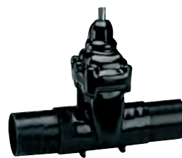
Series 46/70 Gate valve with long spigot ends DN50-600 PN16 Cast steel GP240GH External PUR coating
